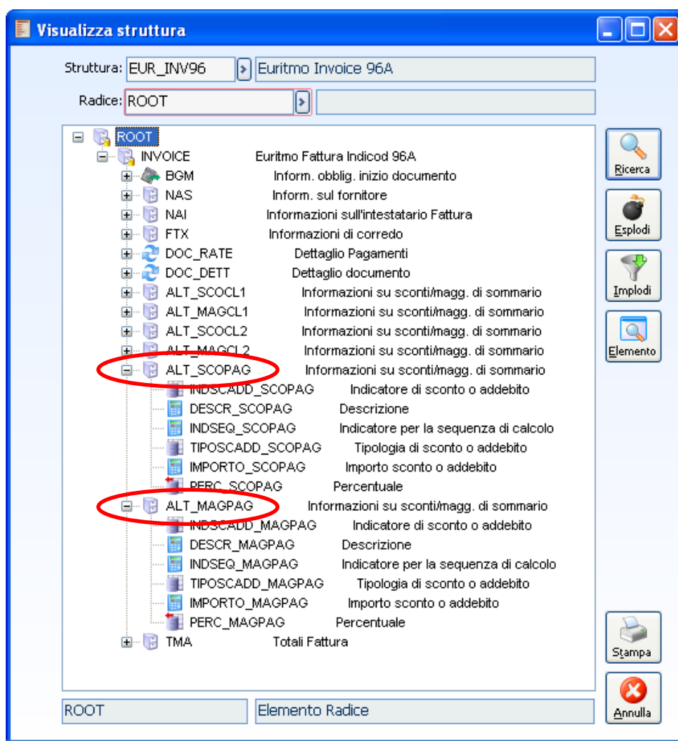
Fig. 1-13 - Treeview
